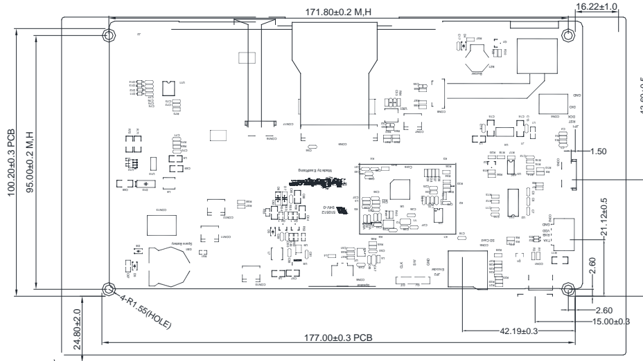
CON2(FFC),CON4 Description
