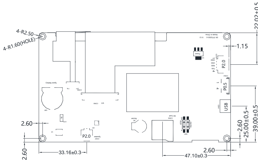
CON2(FFC),CON4 Description
