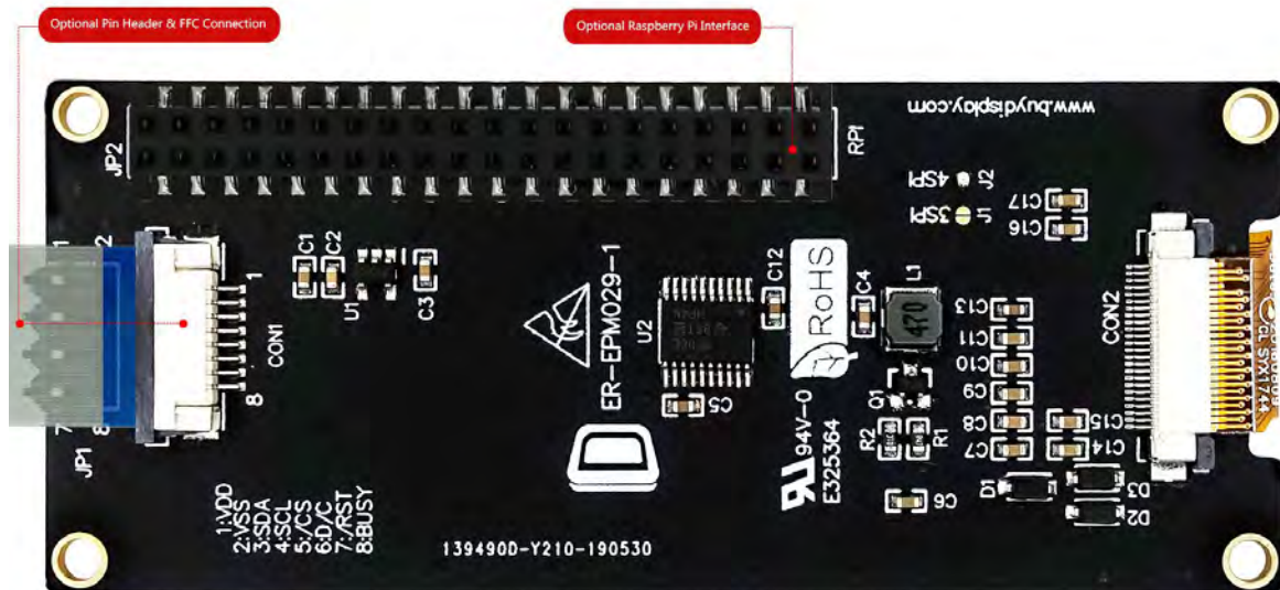
ER-EPM029-2 Bottom View ↓
